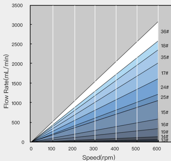
Flow Rate (0.1-600rpm)
